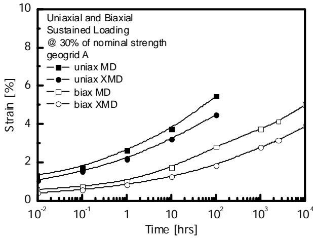
Figure 4 Uniaxial and Biaxial Sustained Loading Tests – Geogrid A
