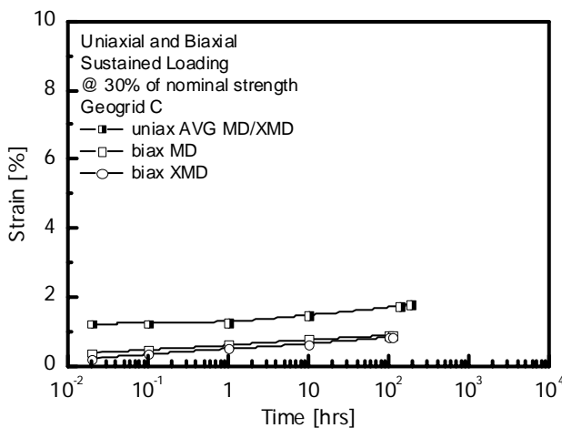
Figure 6 Uniaxial and Biaxial Sustained Loading Tests – Geogrid C
