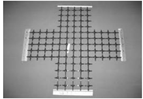
(a) Geogrid with integral junctions
