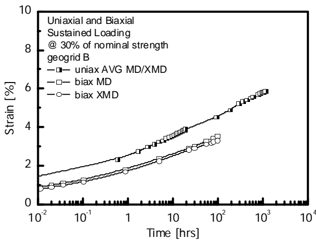
Figure 5 Uniaxial and Biaxial Sustained Loading Tests – Geogrid B
