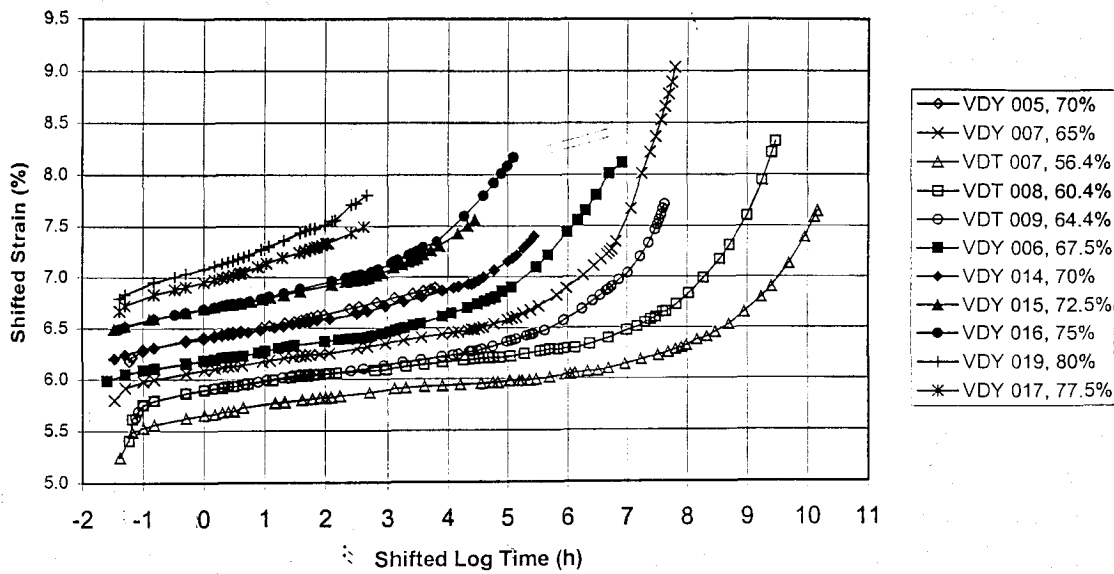
Figure 3. SIM creep curves for all specimens
