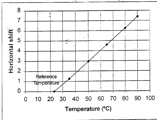
Figure 1. Horizontal shift factors used for specimen VDY 007
