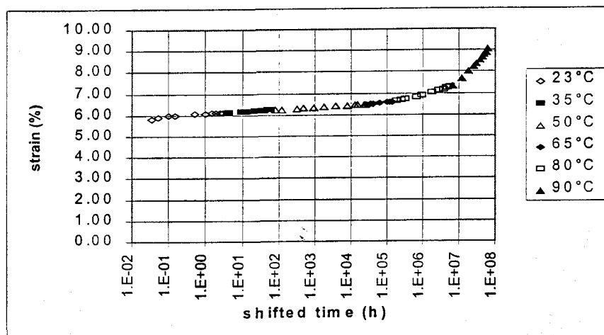
Figure 2. Creep curve for specimen VDY 007
