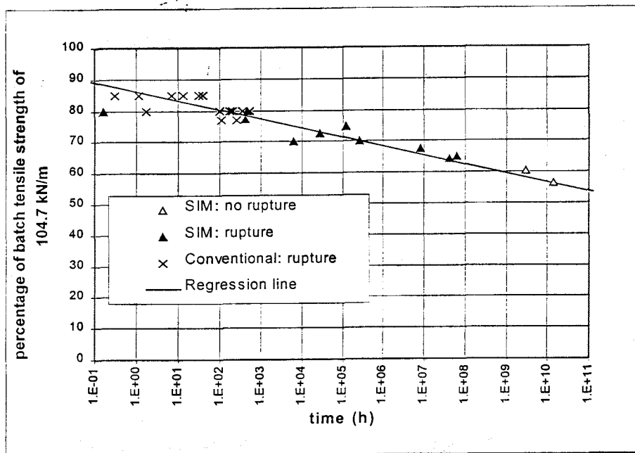
Figure 3. SIM creep curves for all specimens
