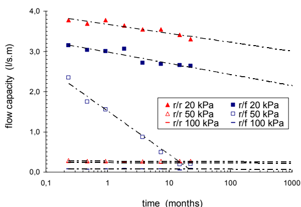
Figure 8. Changes in the flow model in time of a TCT-GCO at load levels between 20 kPa and 100 kPa
