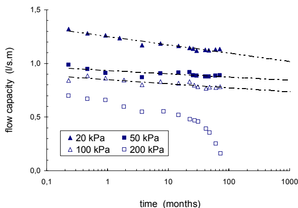
Figure 7. Changes in the flow model in time of a MVM-GCO at different loading at rigid/rigid support
